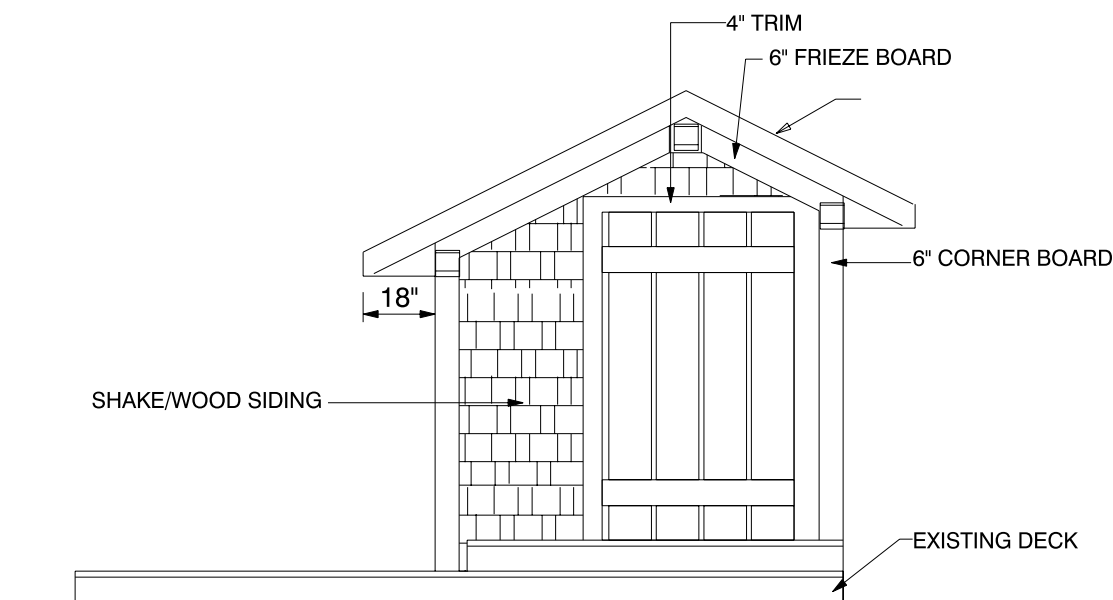
FRONT ELEVATION 1/4" = 1'-0"
