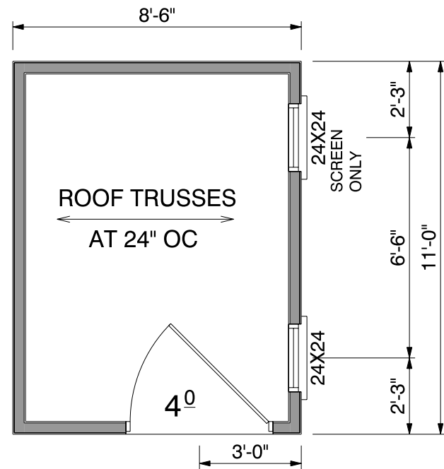
FLOOR PLAN 1/4" = 1'-0"
