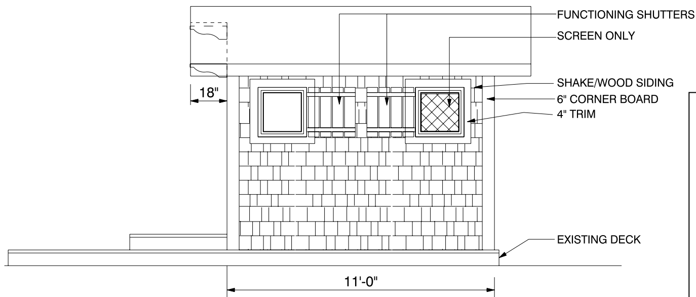
SIDE ELEVATION 1/4" = 1'-0"
