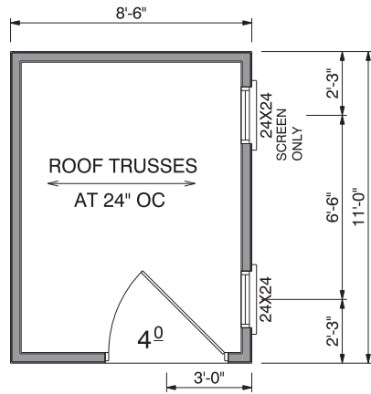
FLOOR PLAN 1/4" = 1'-0"
