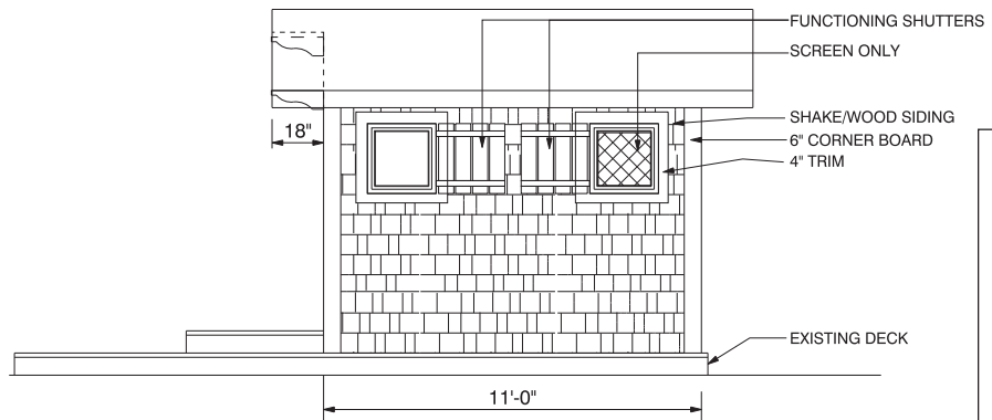
SIDE ELEVATION 1/4" = 1'-0"
