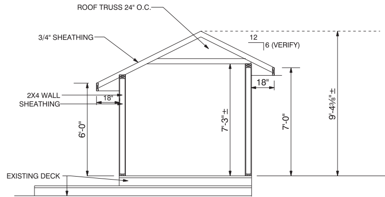
WALL SECTION 1/4" = 1'-0"
