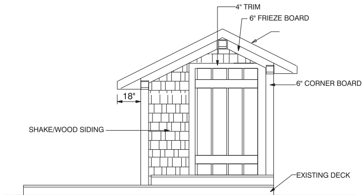
FRONT ELEVATION 1/4" = 1'-0"
