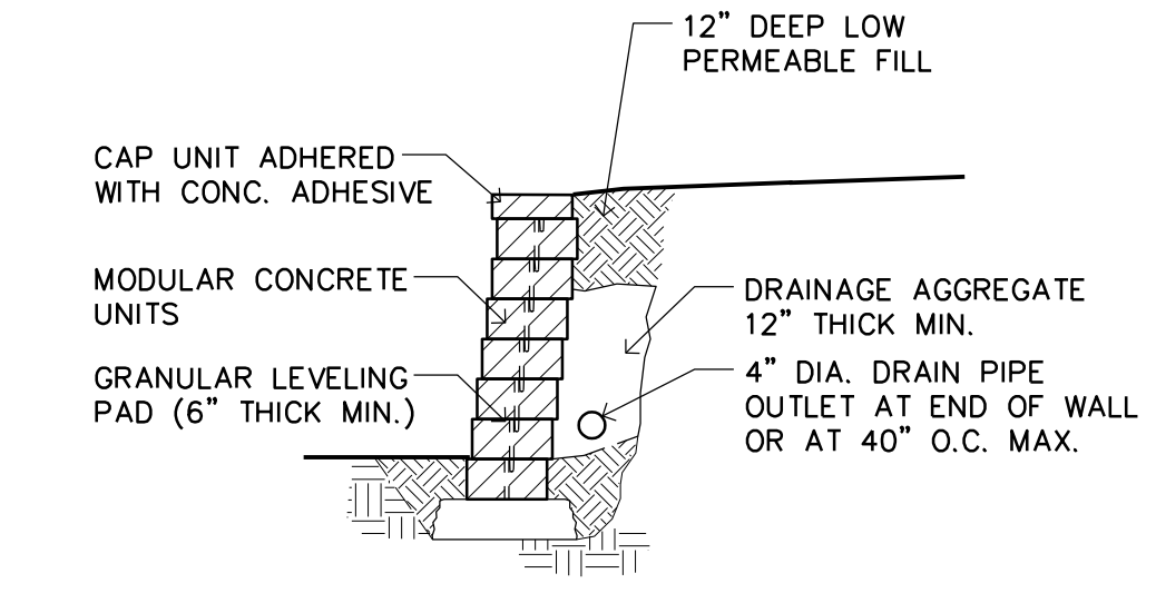
3 RETAINING WALL DETAIL L1 NOT TO SCALE
