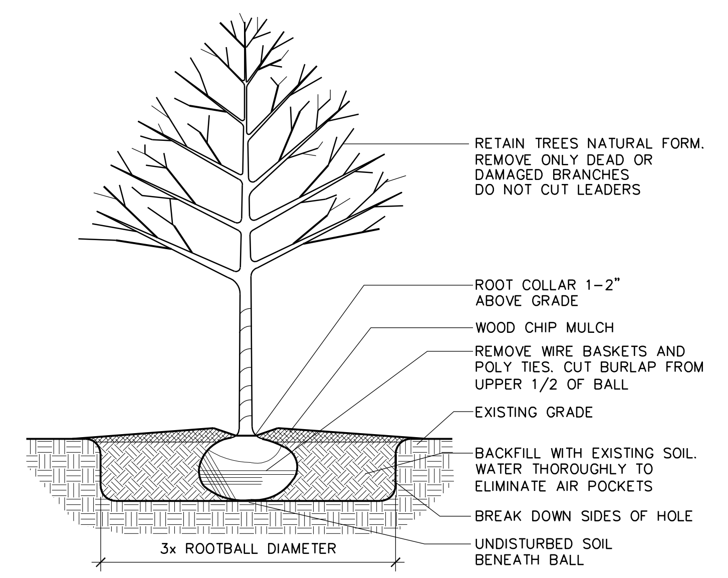
4 TREE PLANTING DETAIL L1 NOT TO SCALE
